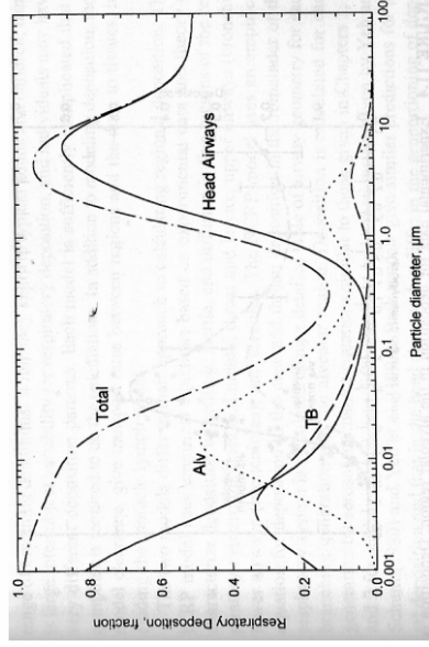
Total and Regional Deposition for Light Exercise (nose breathing) based on ICRP Model
